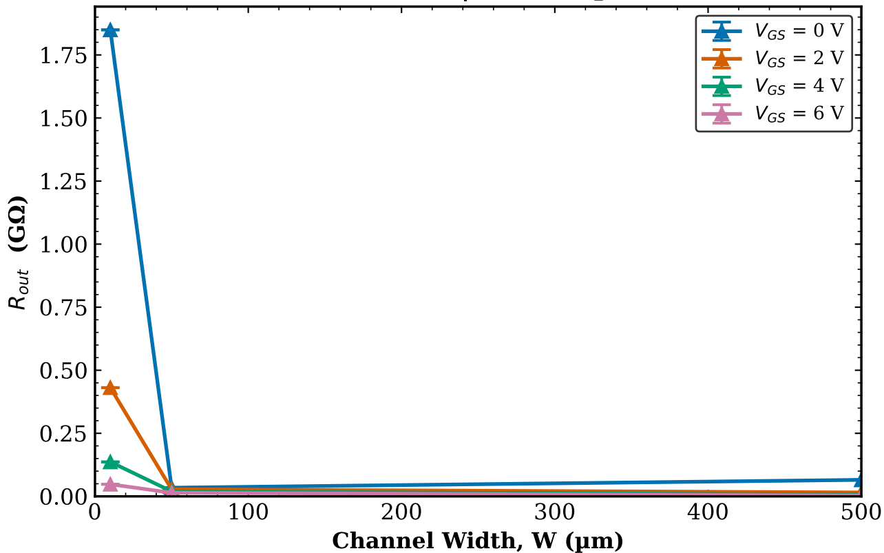
TFT1 Transistor 1 R_{out} vs W | L = 80\text{ }\mu\text{m}
